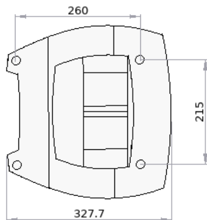
Base type SW (front view)
